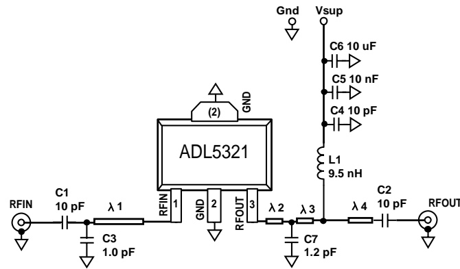
Figure 9. Basic Connections for 3500 MHz to 3850 MHz
