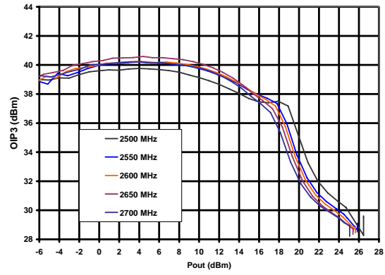
Figure 5. OIP3 vs. Pout and Frequency 2500 MHz – 2700 MHz
